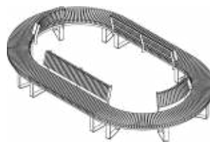
C 5-1-5-1 4677 x 2832 x h875
